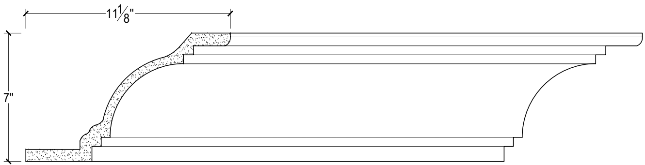
SCALE :4"=1'
