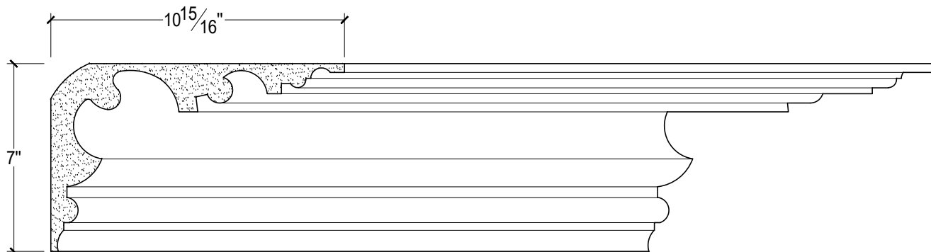
SCALE :4"=1'
