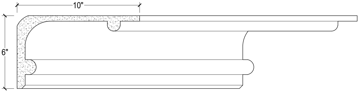
SCALE :3"=1'
