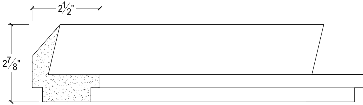
SCALE :2"=1'
