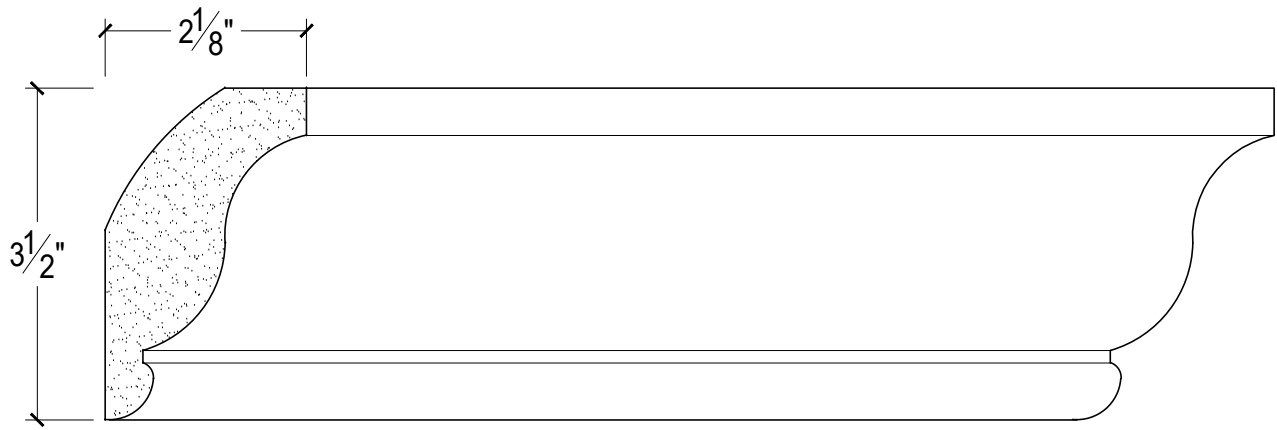
SCALE :2"=1'
