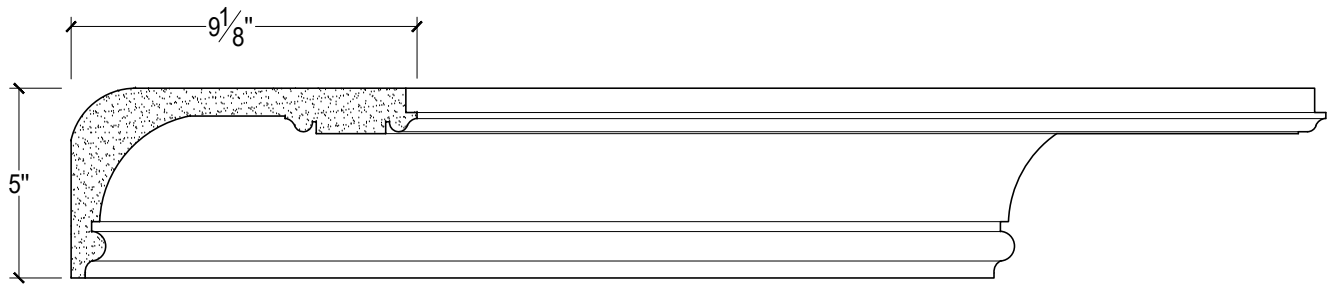
SCALE :4"=1'
