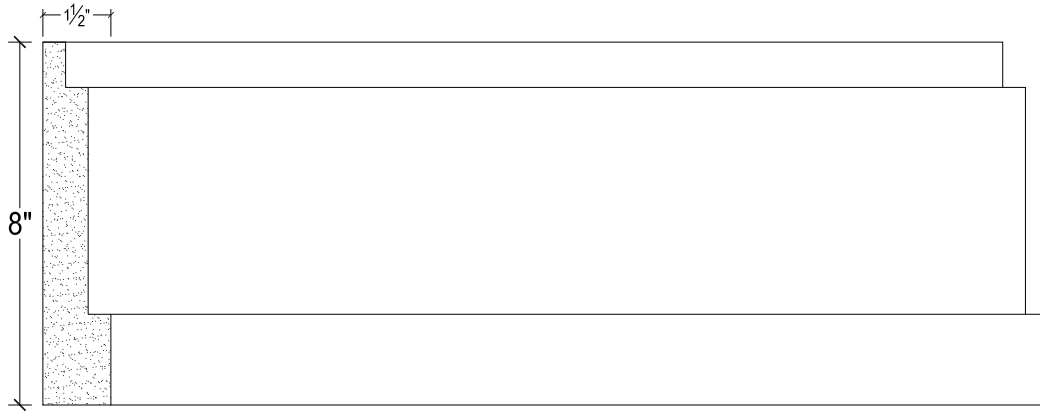
SCALE :3"=1'
