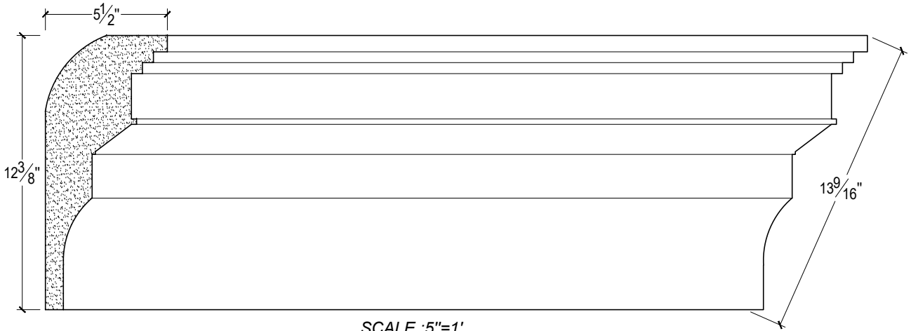
SCALE :5"=1'
