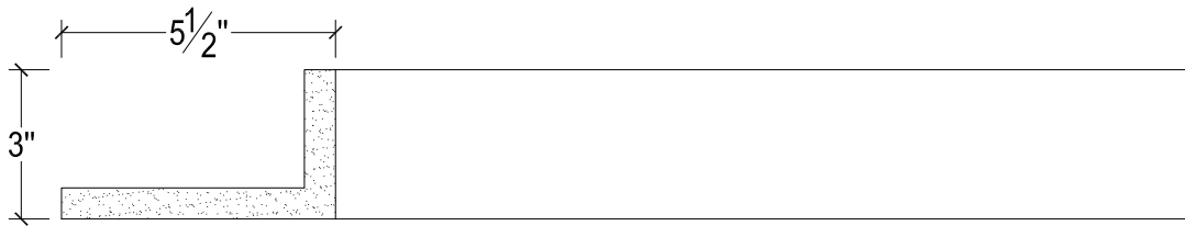
SCALE :3"=1'
