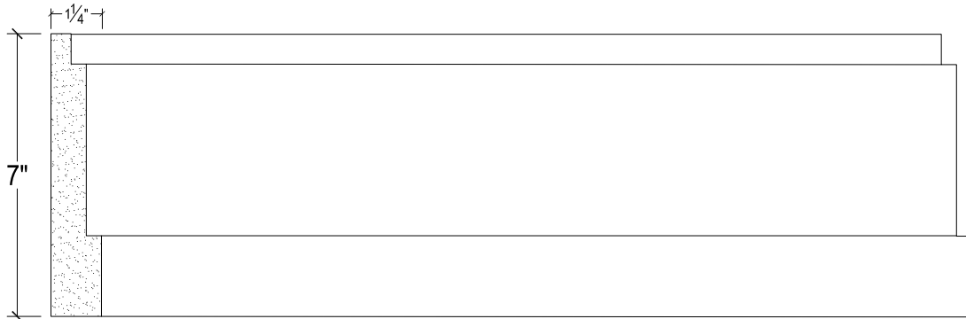
SCALE :3"=1'
