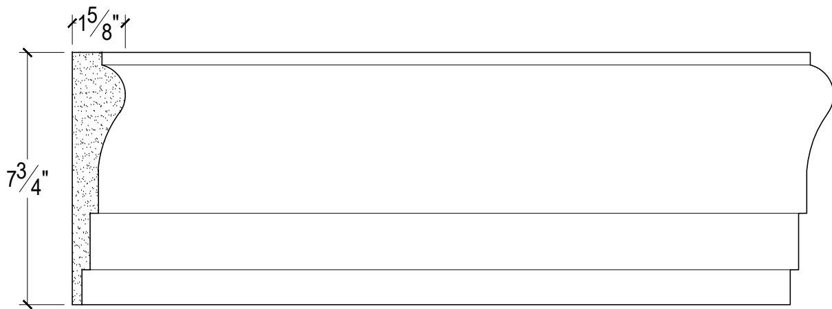
SCALE :3"=1'
