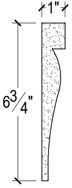
SCALE :3"=1'
