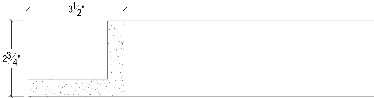
SCALE :2"=1'
