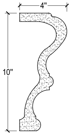
SCALE :4"=1'
