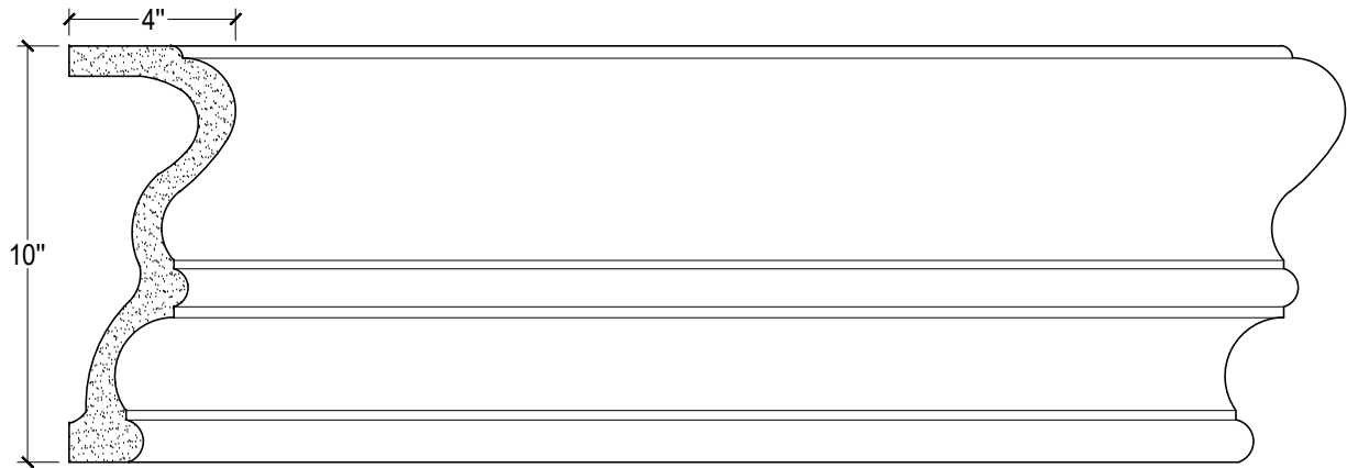
SCALE :4"=1'
