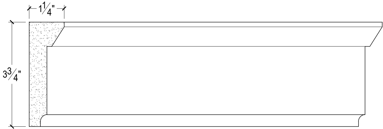
SCALE :2"=1'
