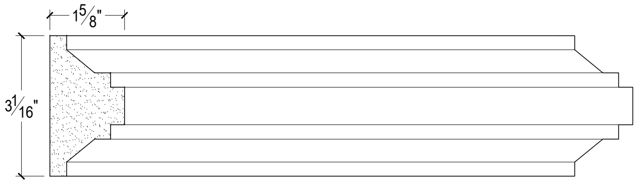
SCALE :2"=1'
