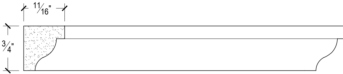
SCALE :1"=1'
