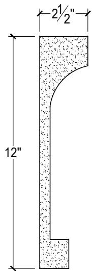
SCALE :4"=1'
