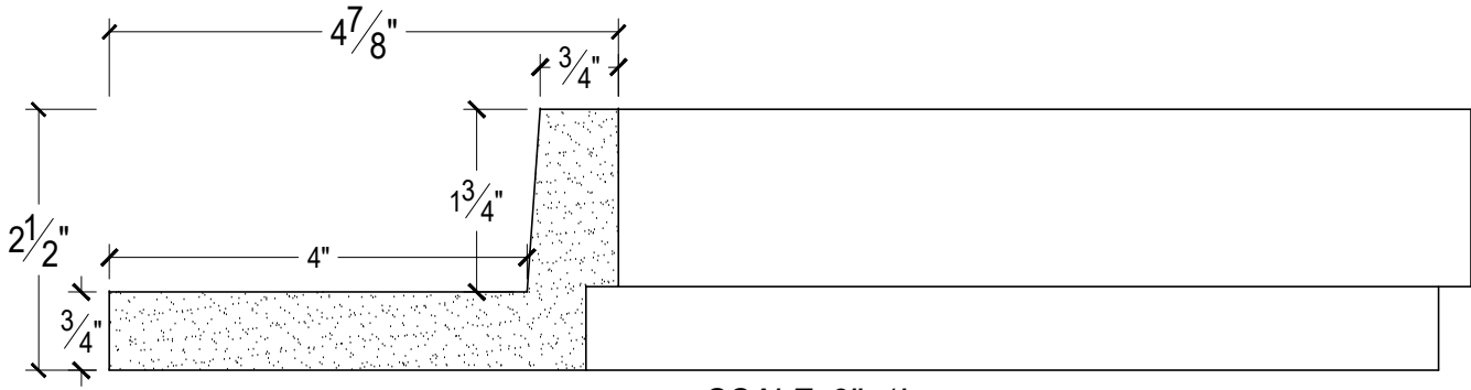
SCALE :2"=1'
