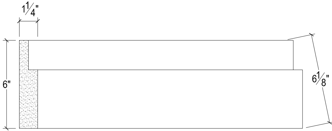
SCALE :3"=1'
