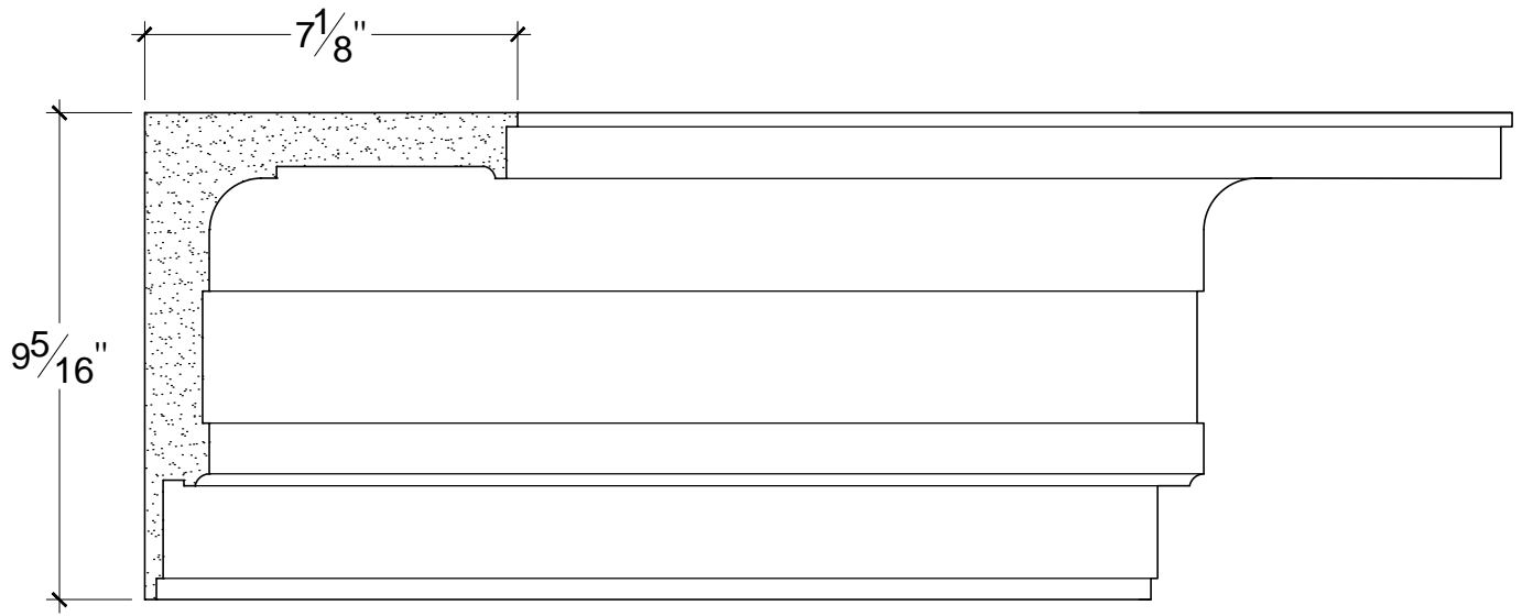
SCALE :3"=1'
