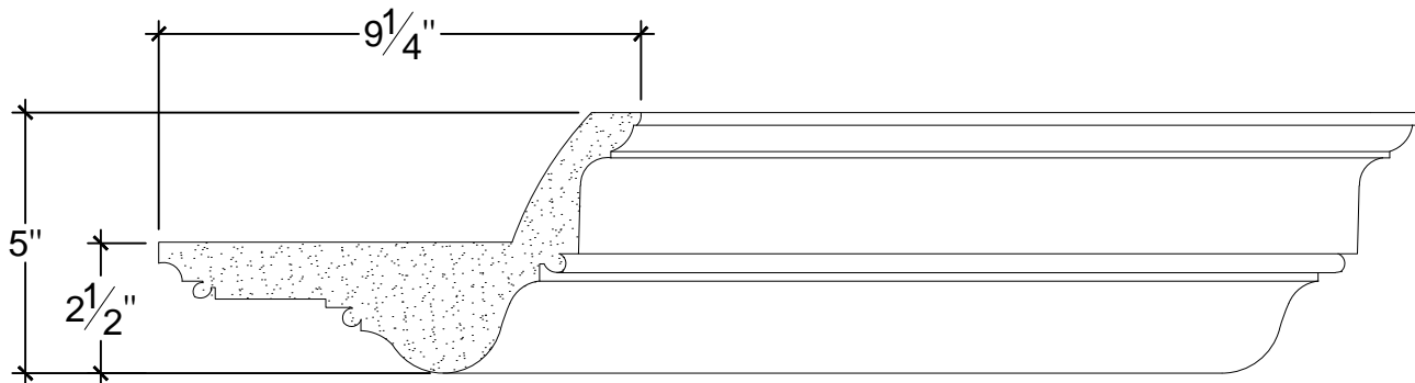
SCALE :3"=1'
